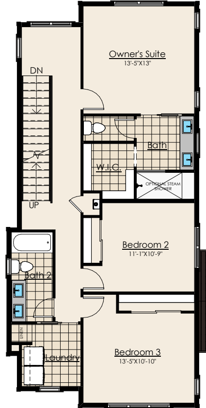
3rd Floor
