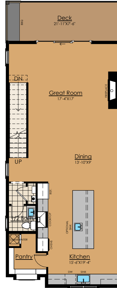
2nd Floor
